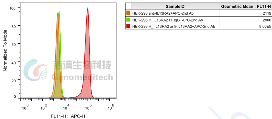
Figure 1 | H_IL13RA2 HEK-293 Cell Line was determined by flow cytometry using Anti-IL13RA2 hIgG1 Antibody(61H8C1) (Genomeditech/GM-86015AB).
